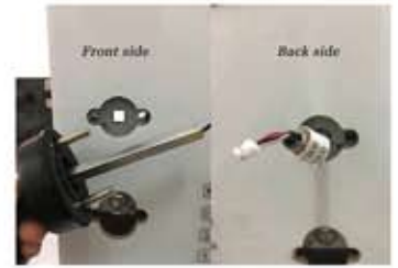
4. Put front handle onto door and get the rod through hole on lock body
